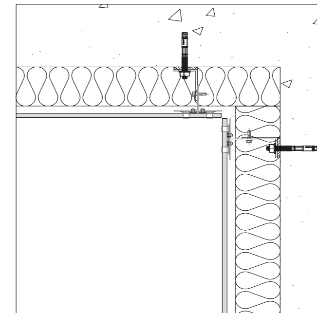
INNER CORNER
